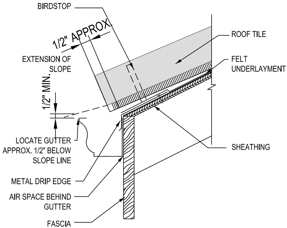
GUTTER FASCIA
