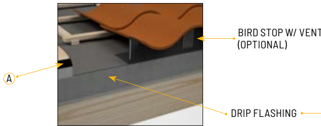
RISER WITH BIRD STOP
